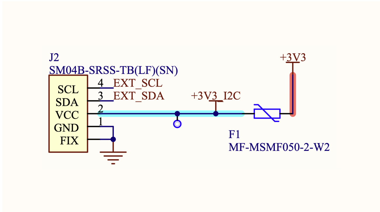
I2C Qwiic connector.
